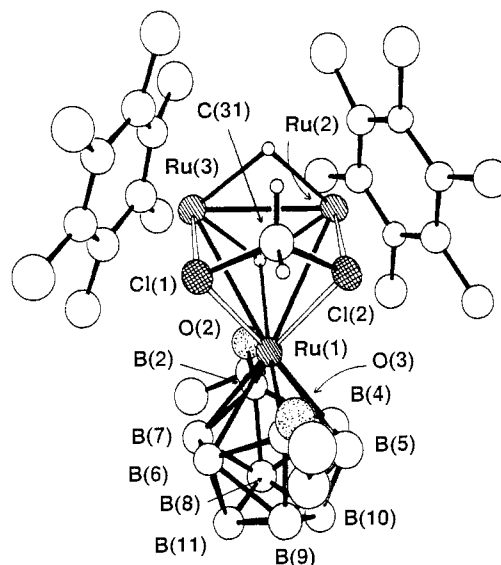
Figure 1. Diagram of the molecule [\{(\eta^6\text{-C}_6\text{Me}_6)_2\text{Ru}_2\text{H}_2(\text{CH}_2\text{Cl}_2)\}\text{RuB}_{10}\text{H}_8(\text{OEt})_2] . Thermal ellipsoids are drawn at the 50% probability level. Ru-C distances average at 2.24 Å; Ru-B distances lie in the range 2.10 (1)-2.36 (1) Å; other dimensions within the closo-type \text{RuB}_{10} cluster are similar to those already reported (ref 4). Proton and ^{11}\text{B} NMR data are as follows (ordered as \delta(^{11}\text{B})/\text{ppm} (relative intensities in parentheses) [with directly bound \delta(^1\text{H})/\text{ppm} in square brackets (relative intensities in parentheses)]): +99.0 (1 B) [OEt], +93.9 (1 B) [OEt], +1.4 (2 B) [+1.78 (2 H)], -1.3 (3 B) [+3.59 (1 H), +1.41 (2 H)], -4.0 (1 B) [+2.61 (1 H)], -6.5 (2 B) [+0.61 (2 H)]; also \delta(^1\text{H}) ( \eta^6\text{-C}_6\text{Me}_6 ) +2.17 ppm; \text{CD}_2\text{Cl}_2 solution at 297 K.
