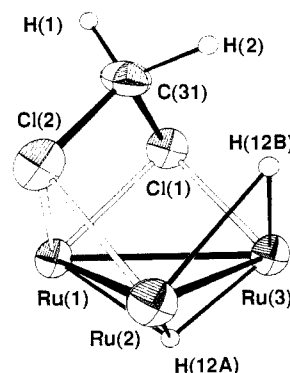
Figure 2. Diagram showing the binding of the dichloromethane molecule to the \text{Ru}_3 triangle in [\{(\eta^6\text{-C}_6\text{Me}_6)_2\text{Ru}_2\text{H}_2(\text{CH}_2\text{Cl}_2)\}\text{RuB}_{10}\text{H}_8(\text{OEt})_2] . Thermal ellipsoids are drawn at the 50% probability level. Selected interatomic distances (angstroms) and angles (degrees) are as follows: Ru(1)-Ru(2), 3.100 (1); Ru(2)-Ru(3), 2.869 (1); Ru(1)-Ru(3), 3.106 (1); Ru(1)-Cl(1), 2.403 (3); Ru(1)-Cl(2), 2.396 (2); Ru(2)-Cl(2), 2.315 (3); Ru(3)-Cl(1), 2.319 (3); Ru(1)-H(12A), 2.19 (8); Ru(2)-H(12A), 1.92 (7); Ru(3)-H(12A), 1.88 (7); Ru(2)-H(12B), 2.20 (7); Ru(3)-H(12B), 2.20 (7); C(31)-Cl(1), 1.803 (9); C(31)-Cl(2), 1.827 (9); Ru(1)-Cl(1)-Ru(3), 82.2 (1); Ru(1)-Cl(2)-Ru(2), 82.3 (1); Cl(1)-C(31)-Cl(2), 102.4 (5). Proton NMR data are as follows: \delta(^1\text{H}) (H(1)) +2.49 ppm (d), \delta(^1\text{H}) (H(2)) +4.89 ppm (ddd), \delta(^1\text{H}) (H(12A)) -14.74 ppm (dd), \delta(^1\text{H}) (H(12B)) -22.40 ppm (dd); ^2J(\text{H}(1)-\text{H}(2)) 10.1 Hz, ^4J(\text{H}(2)-\text{H}(12A)) 1.2 Hz, ^4J(\text{H}(2)-\text{H}(12B)) 5.3 Hz, ^2J(\text{H}(12A)-\text{H}(12B)) 4.9 Hz.
